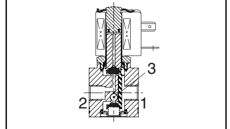
U function (stainless steel body)
